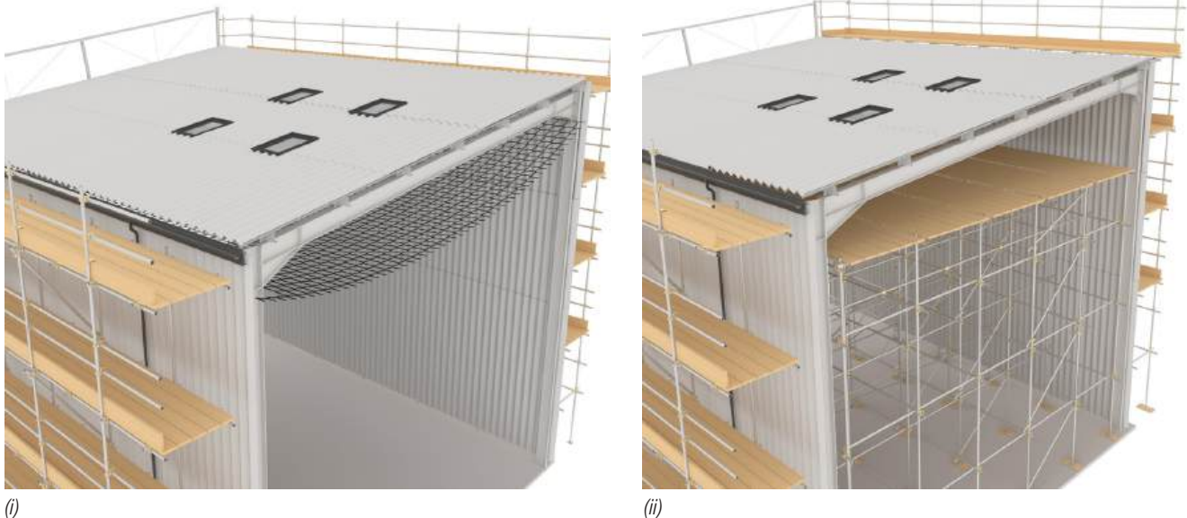
Figure 10: Cross-sections showing examples of collective fall arrest below fragile surfaces, (i) fall arrest safety netting and (ii) birdcage protection deck.
