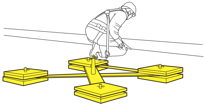
Figure 55: A selection of special connectors and anchor devices.
