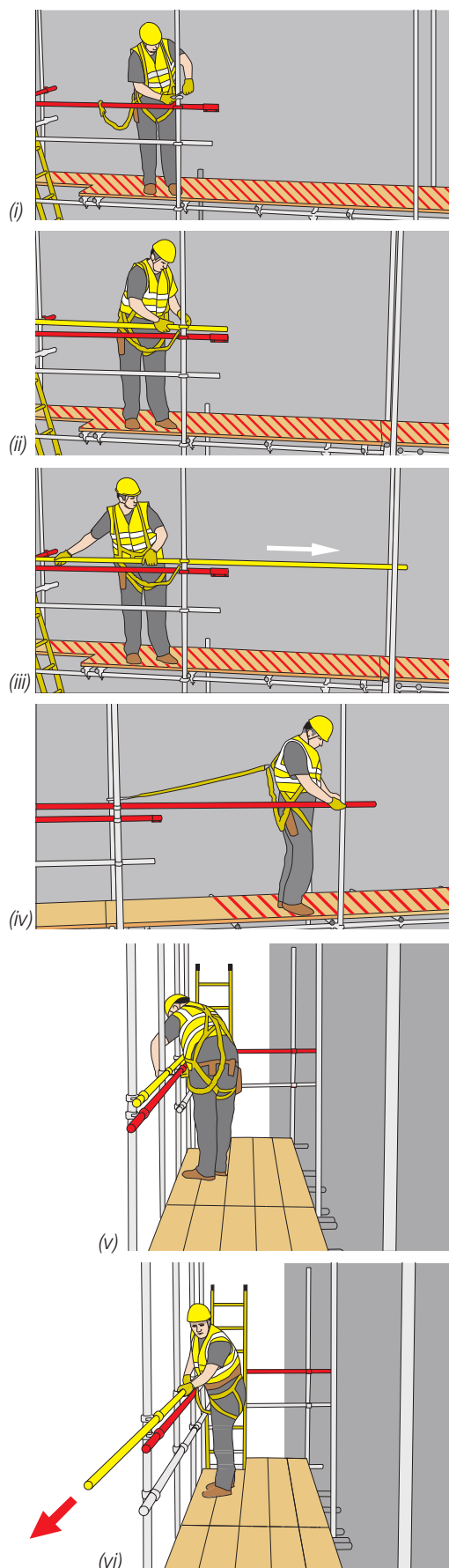
Figure 37: Shows a sequence of installing a tube and fitting advanced guardrail horizontally.
