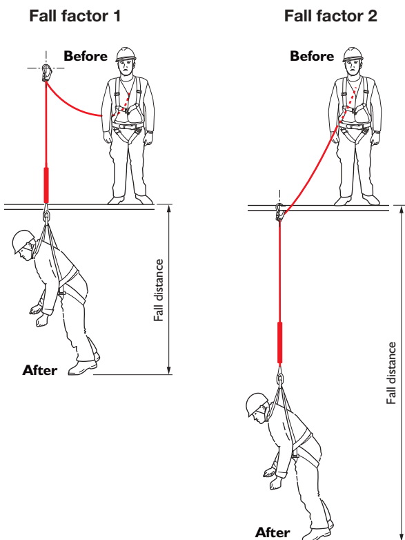
Figure 44: Fall factors.
