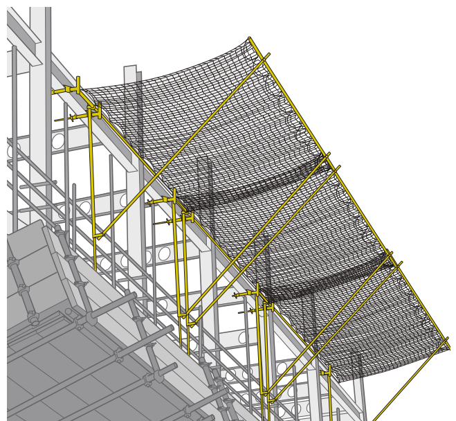
Figure 93: Safety net fan system provides protection for erecting temporary edge protection.
