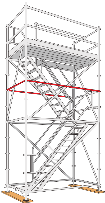
Figure 65: Typical proprietary system scaffold stairway
