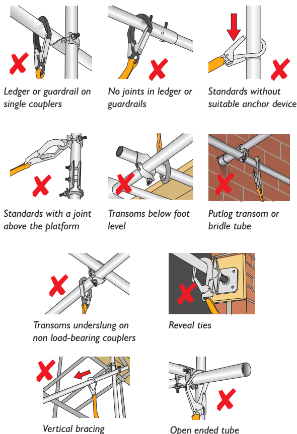
Figure 53: Examples of unsuitable anchor points.
