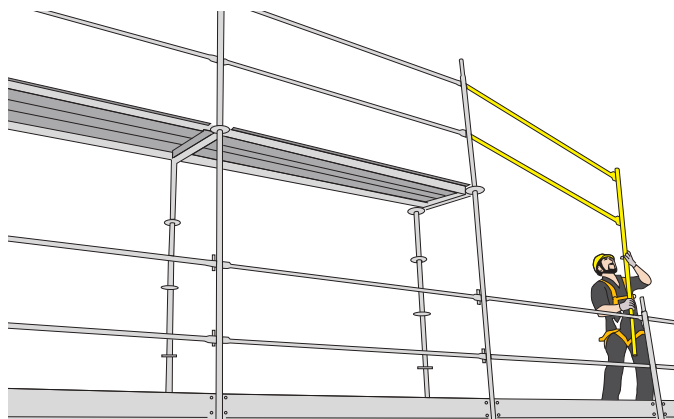
Figure 32: An example of an integrated advanced guardrail system for a proprietary scaffolding system.
