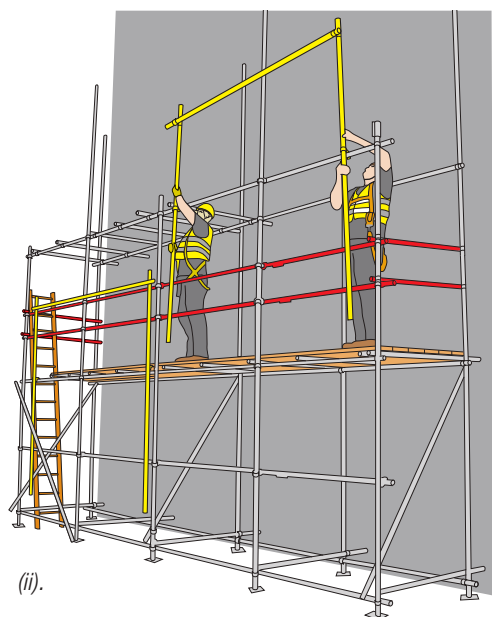
Figure 36: AGS frame constructed on the ground and fixed to the base lift. (i). Releasing the guardrail from the ledger. (ii). Raising the guardrail to the next level.
